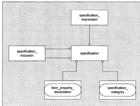
Figure 7. Entity diagram describing the module instances
