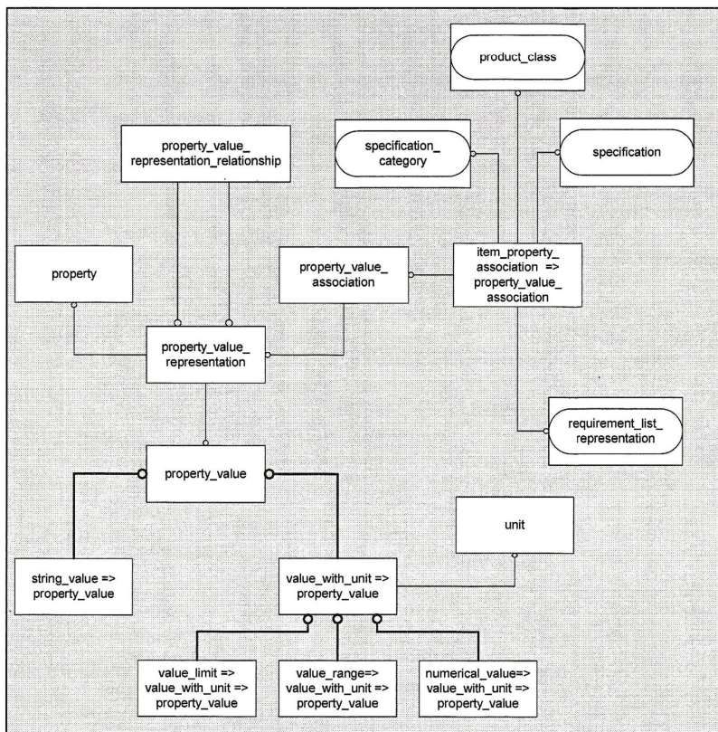
Figure 5. Entity diagram describing the property value
