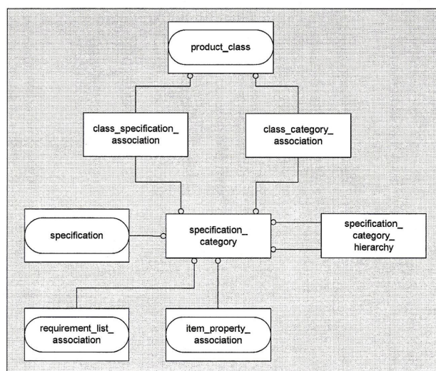
Figure 6. Entity diagram describing the classification of modules
