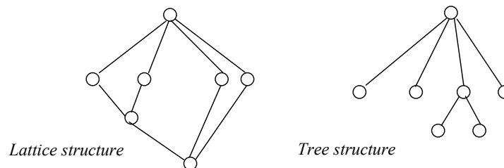
Figure 2. Tree and lattice structure
